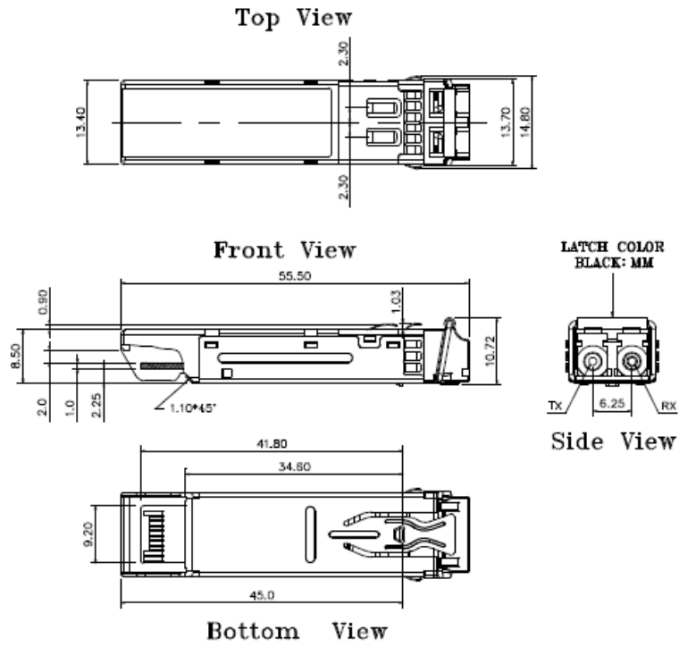
(例: 2心版: SPS-2381W-C530-046G)
